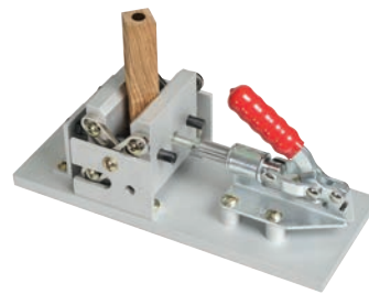
CARBATEC Quick Action Self-Centring Pen Blank Drilling Jig
