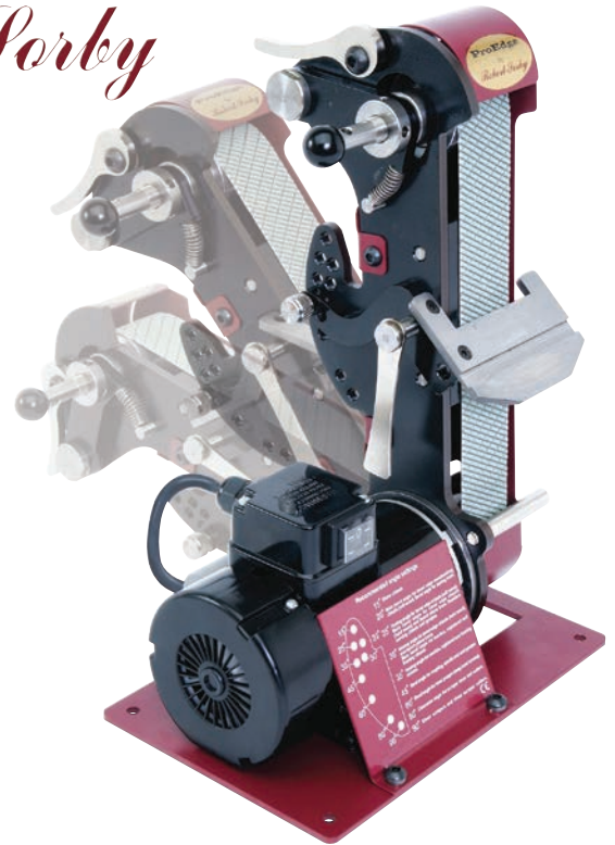
ROBERT SORBY ProEdge Deluxe Sharpening System Part No. RSB-WPED01D
