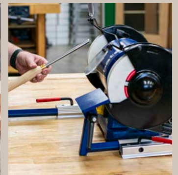
CARBATEC Spindle and Gouge Sharpening System Part No. CT-SGSS-01
