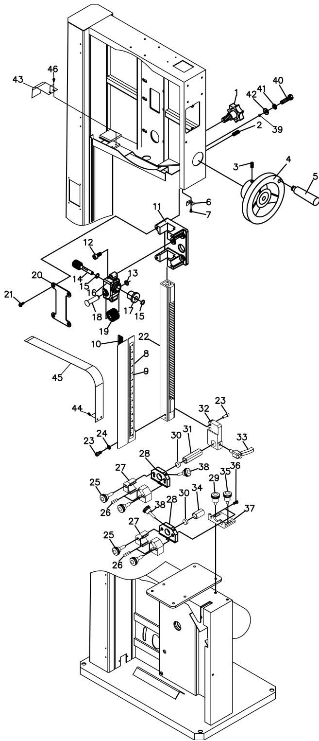
Upper and Lower Blade Guides Assembly
