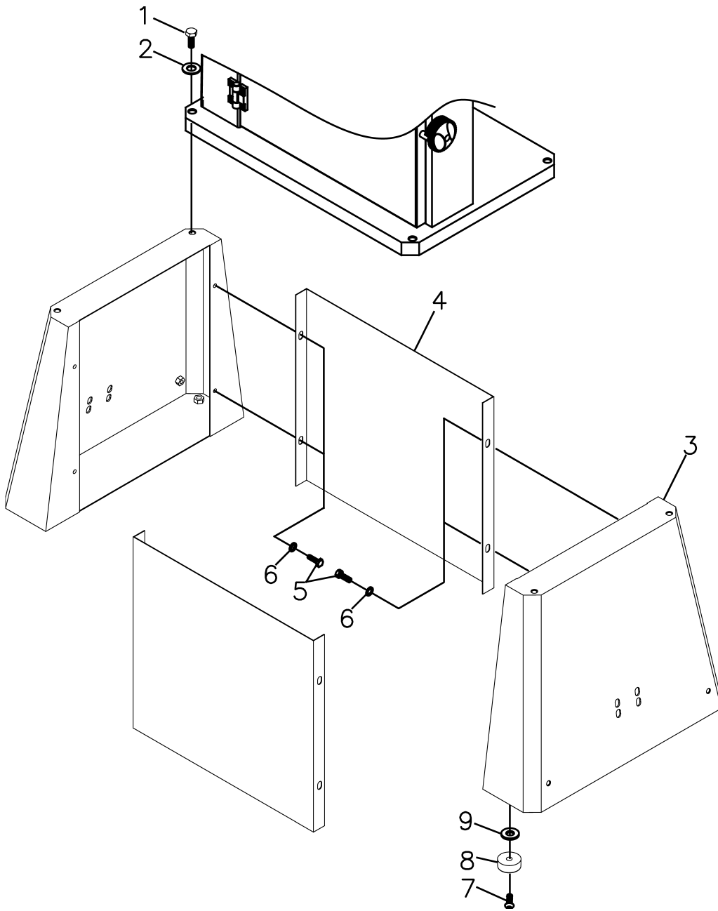
Stand Assembly
