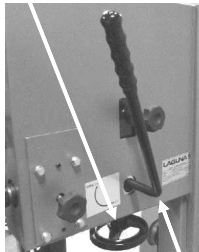
Quick action blade tension lever (activated)
