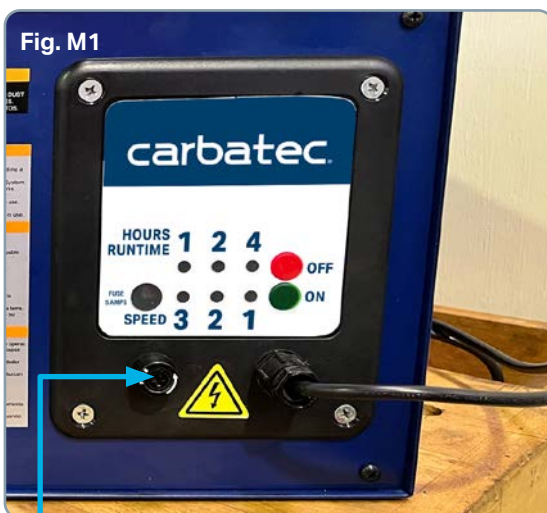
FUSE HOLDER
