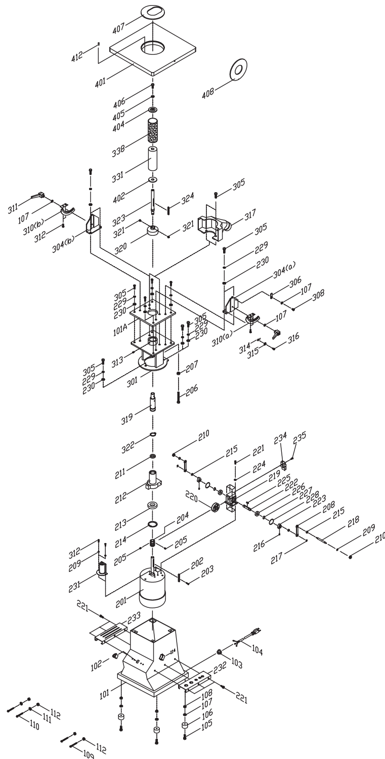
Carbatec Benchtop Oscillating Spindle Sander SPS-375P
