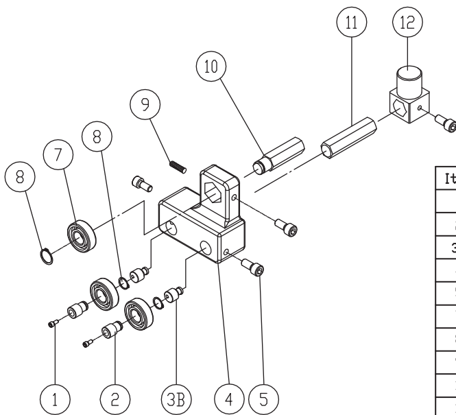
MODEL NO. : 17 Inch Band Saw PART NO. : AB135091 UPPER BLADE GUIDE SUPPORT (ASM)
