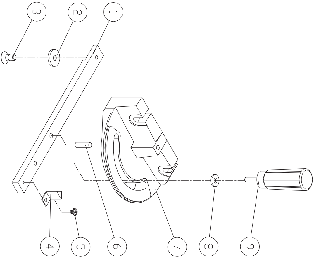
MODEL NO.: 17 Inch Band Saw PART NO.: AB198101 MITER GAUGE ASS'Y
