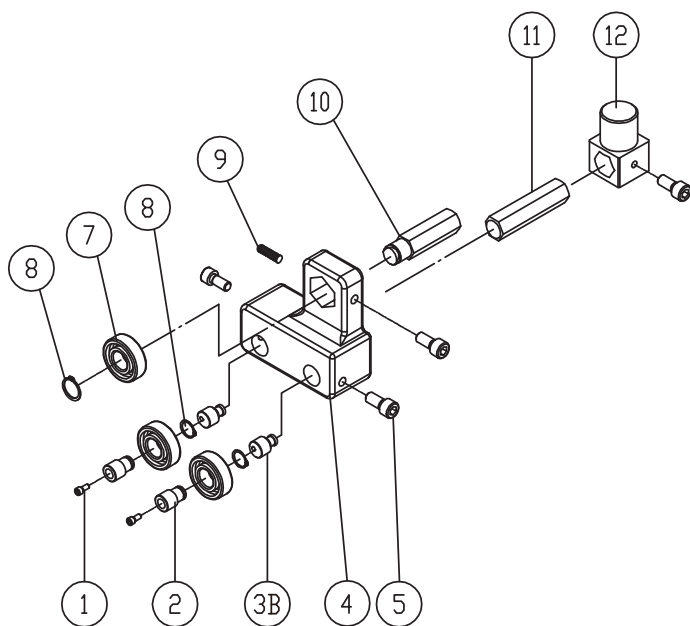
MODEL NO.: OPTIONAL PART NO.: AB135091 UPPER BLADE GUIDE SUPPORT (ASM)
