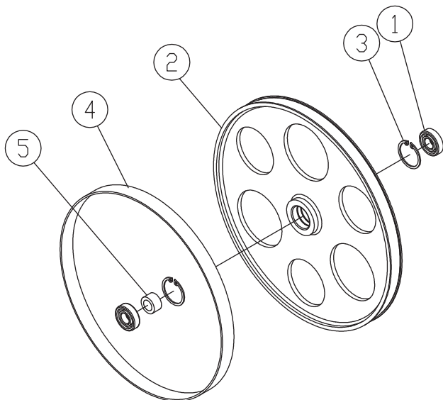
MODEL NO.: OPTIONAL PART NO.: AB136024T UPPER WHEEL
