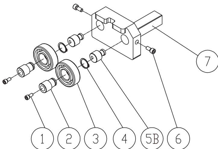
MODE NO.: OPTIONAL PART NO.: AB135093A LOWER BLADE GUIDE SUPPORT (ASM)
