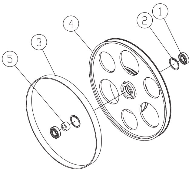
MODEL NO.: OPTIONAL PART NO.: AB136022T LOWER WHEEL ASM
